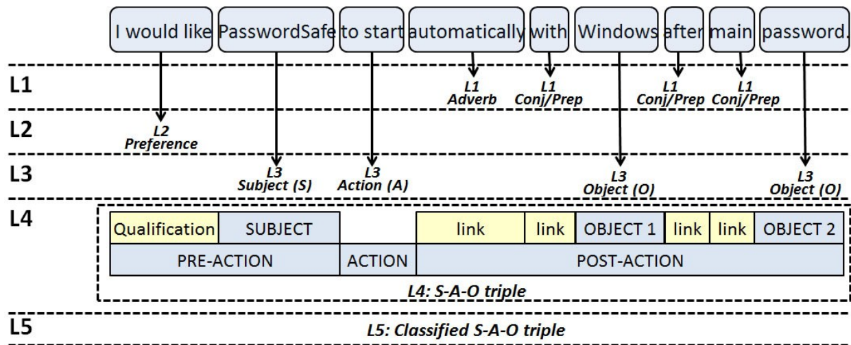
Figure 3. Text tagged with the grammar-based requirements ontology.
